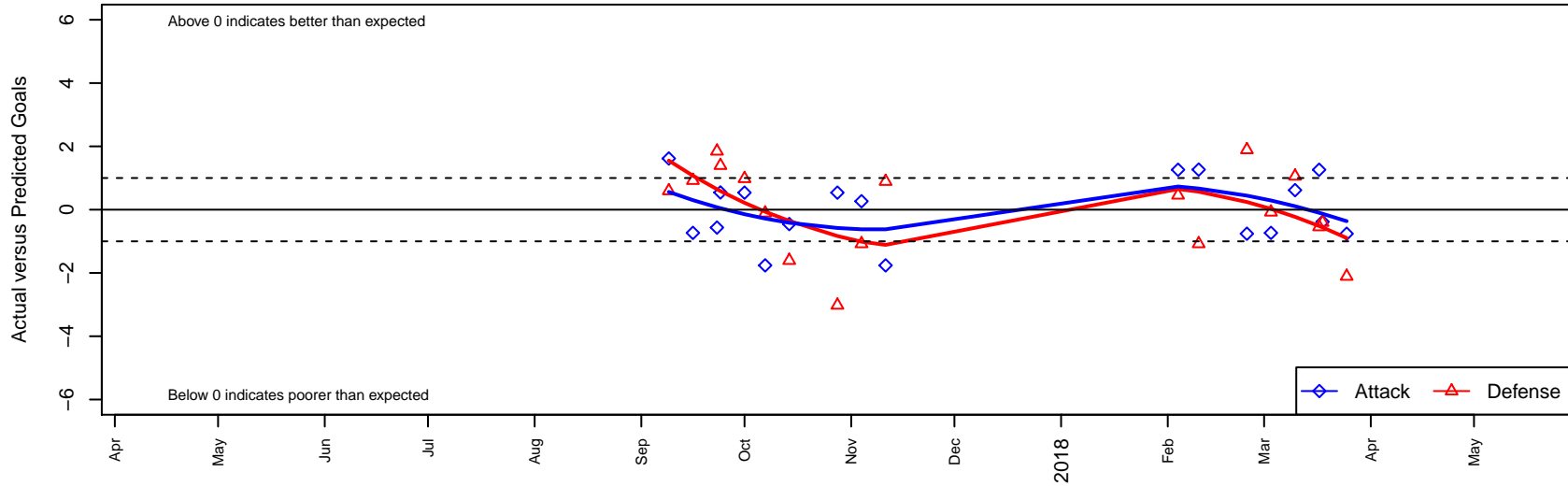
NPSA Titans Navy G04 Dots are actual minus expected GF (blue circles) and GA (red triangles). Blue line is smoothed change in attack strength. Red is smoothed change in defense strength.
